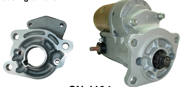
SN-1104 2.0kw, CW, 9T OEM:128000-104, CATERPILLAR:3E5130
