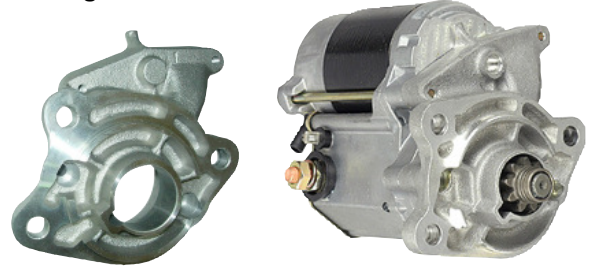
SN-0982 1.4kw, CW, 9T OEM:028000-982, CATERPILLAR:3E5128
