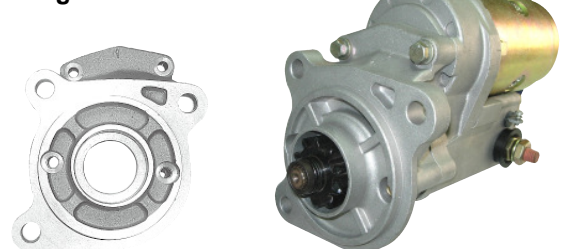
SN-1737R 1.4kw, CW, 10T OEM:028000-823, CATERPILLAR:3T5649
