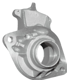
SN-1100 4.5kw, CW, 11T OEM:128000-100, KOMATSU:600-813-3240
