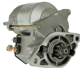
SN-2656 1.4kw, CW, 9T OEM:228000-632, KUBOTA:16235-63010
