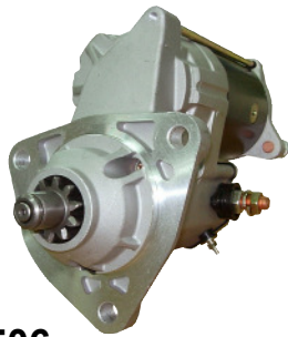
SN-19506 5.0kw, CW, 10T, R5 Type OEM:428000-543
